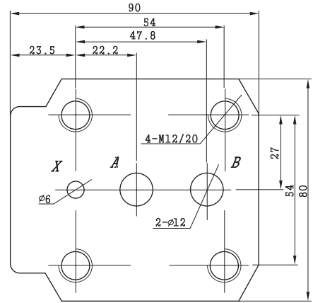
Subplate mounting
